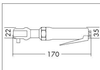
Dimensions of 1/4" and 3/8" version
