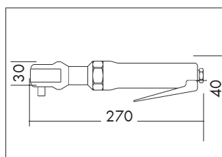
Dimensions of 1/2" version
